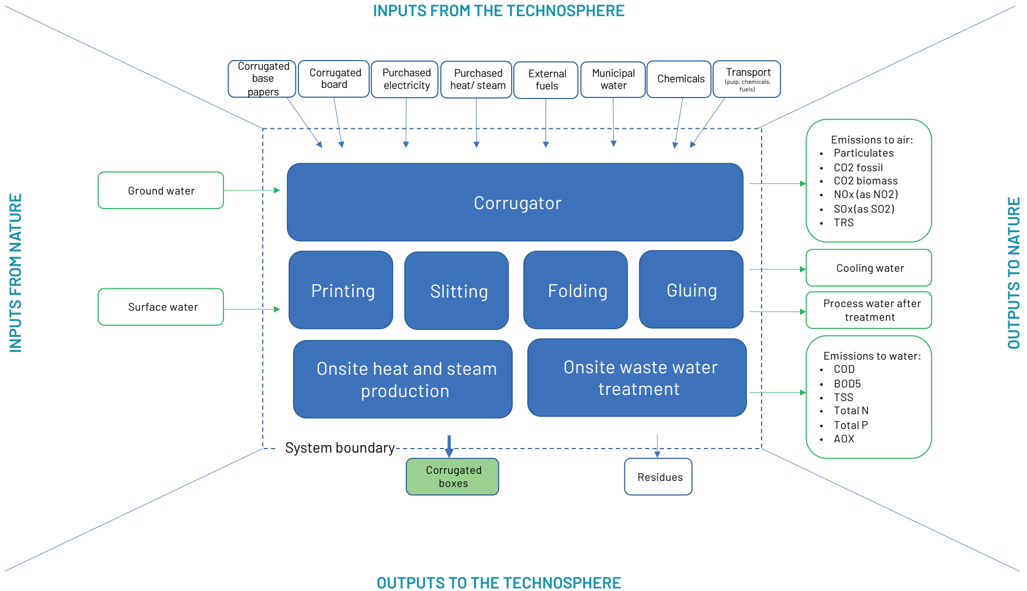
Figure 10 Gate-to-gate system boundaries – production of corrugated board and corrugated boxes
