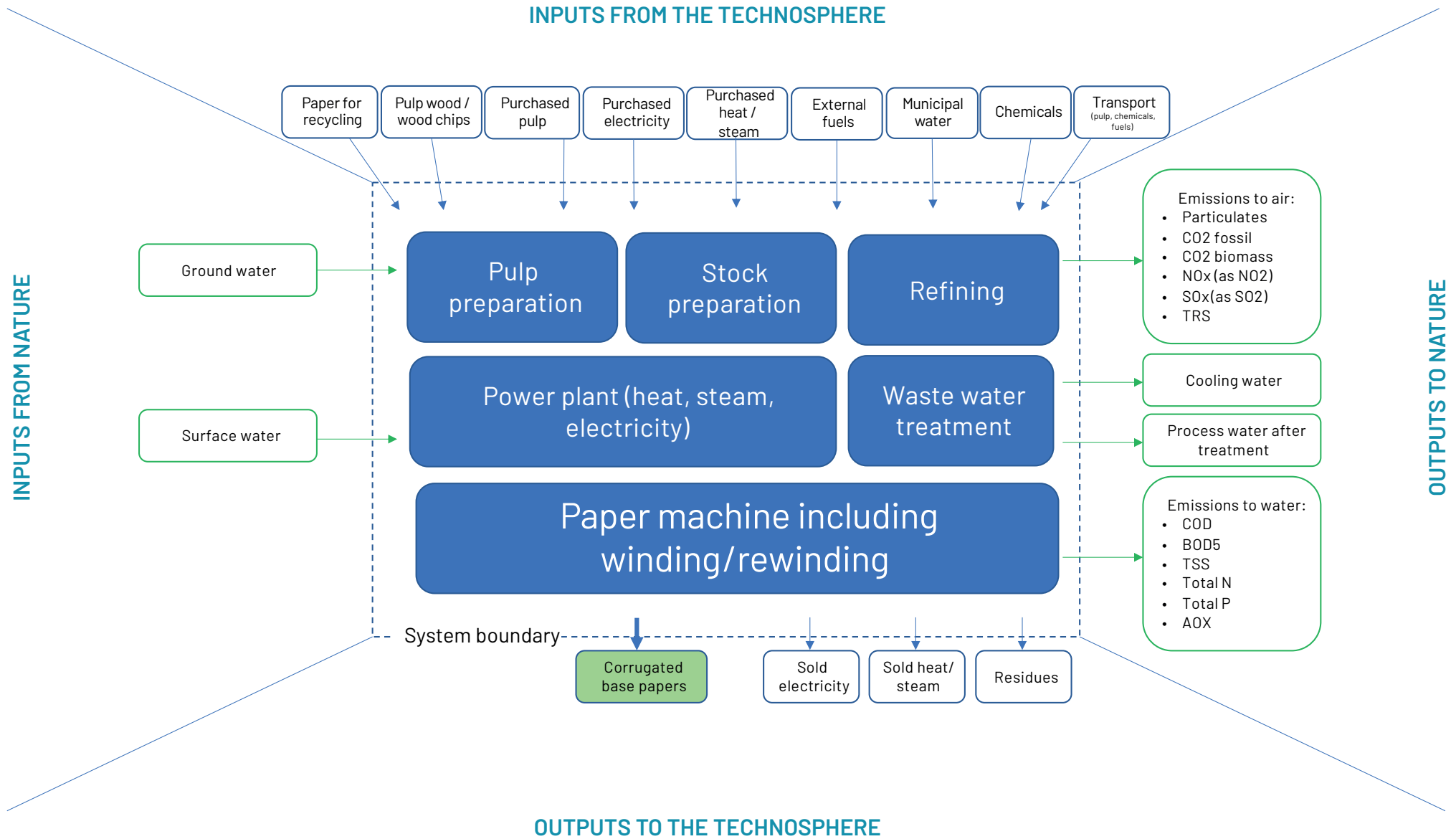
Figure 9 Gate-to-gate system boundaries – production of corrugated base paper
