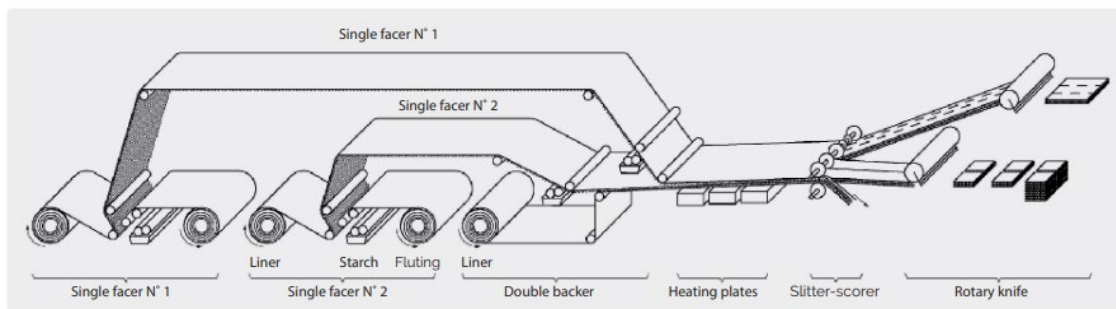
Figure 4: Corrugated board production
