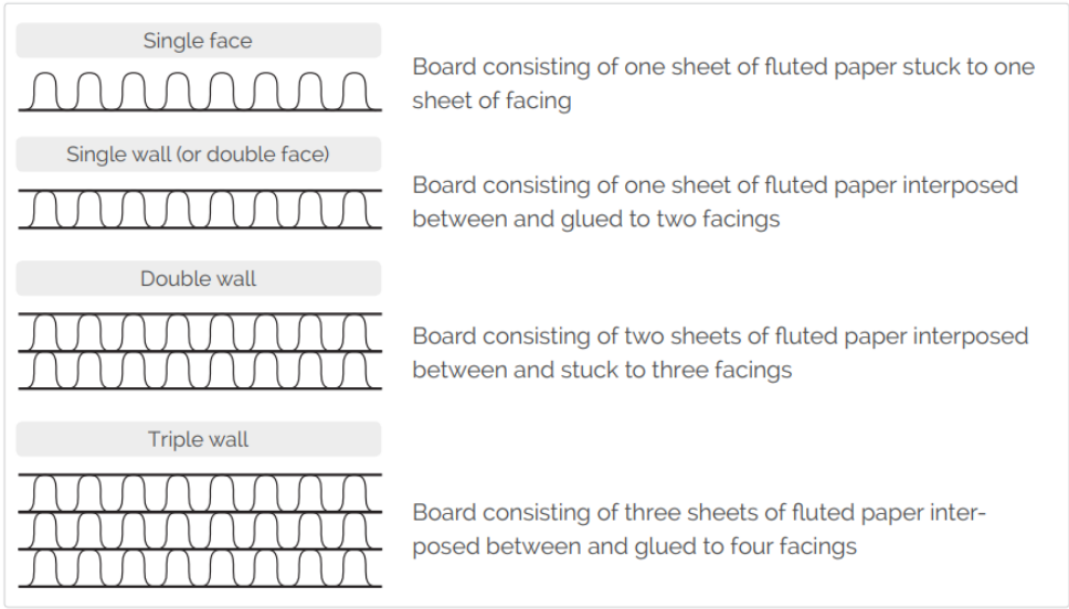
Figure 2: Corrugated board constructions
