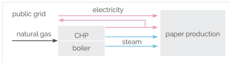
Figure 12 CHP, Combined heat and power generation
