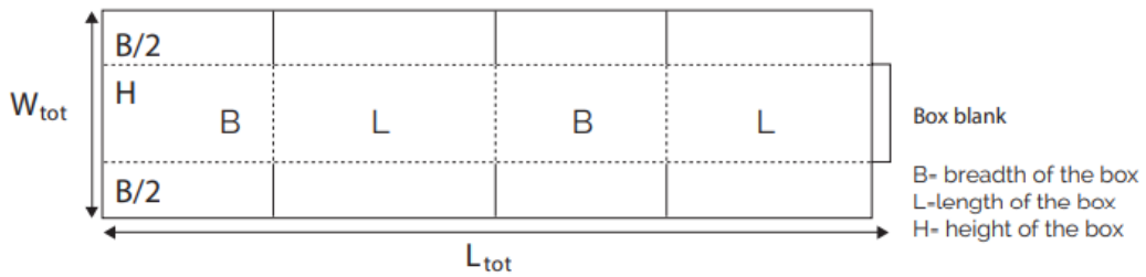
Figure 6 Box blank example
